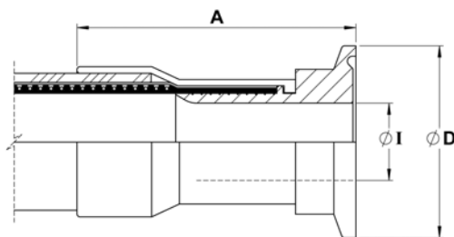
MINI-SANITARY TRICLAMP (TRICLOVER) FITTINGS
