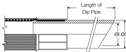
FIXED DIP PIPE (STRAIGHT)
